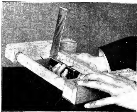
Fig. 219—Testing with Trysquare
